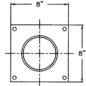
4" FPT PIPE COUPLING PART NO. C400E- ENAMELED STEEL C400S- STAINLESS STEEL
