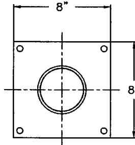
3" FPT PIPE COUPLING PART NO. C300E- ENAMELED STEEL C300S- STAINLESS STEEL
