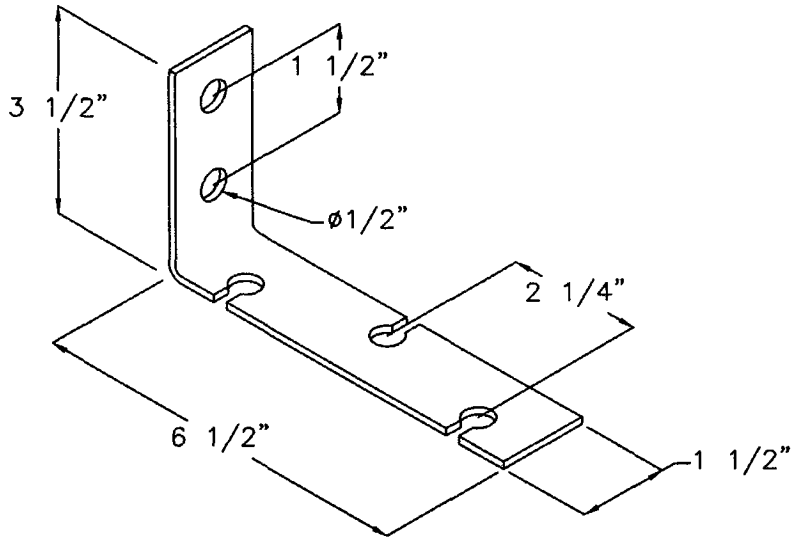
SSFB3 - Stainless Steel Float Bracket With (3) 3/8" Cord Grips
