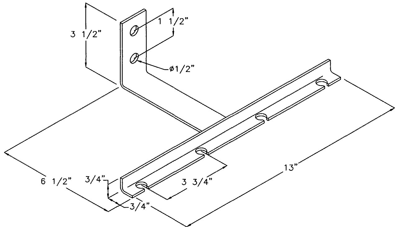
SSFB413 - Stainless Steel Float Bracket With (4) 3/8" Cord Grips
